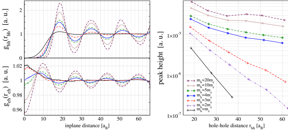
Figure 4. Left: hole-hole (top) and e-h (bottom) pair distribution functions for a macroscopic bilayer with the mass ratios M = 1, 3, 4, 5, 10, 20 (the maxima increase with increasing M ). Note the alternating location of maxima and minima of g_{hh} and g_{eh} . Right: decay of the amplitude of the maxima and minima of the hole correlations ( |g_{hh} - 1| ) for the seven mass ratios. From [34].
