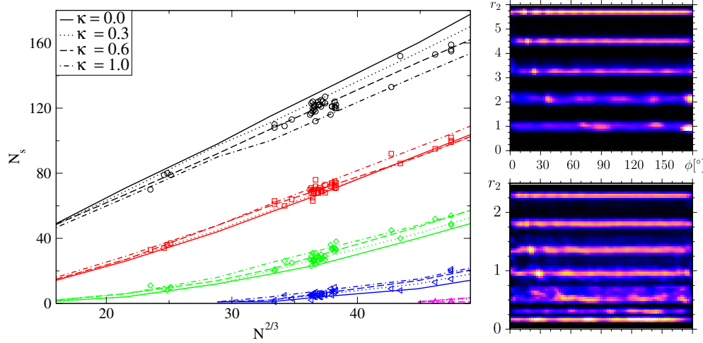
Figure 1. Left: experimental (symbols) and simulation (lines) shell populations N_s of harmonically confined dust crystals as a function of the system size N^{2/3} . The simulation results (lines) are obtained for different screening parameter \kappa and show that the particles are redistributed from the outer shell to inner shells with increased screening. From [7]. Right: three particle correlation function for 3D plasma crystals with N = 500 , \Gamma = 1000 , and screening parameter \kappa = 0 (top) and \kappa = 3.8 (bottom). White (black) denotes areas of high (low) correlation; r_1 is integrated out.
