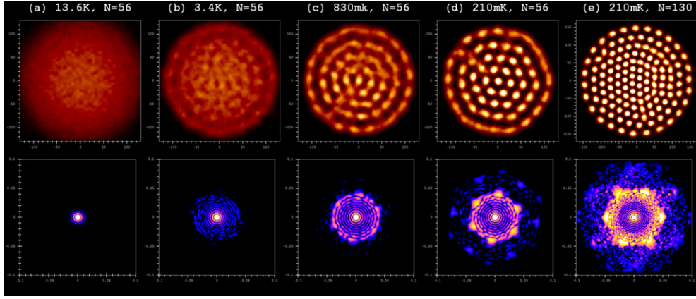
Figure 2. Temperature-driven phase transition of (a)–(d) N_x = 56 , (e) N_x = 130 harmonically trapped indirect excitons in a 30 nm wide ZnSe-based quantum well. Top row: density plots for the temperatures: 13.6 K, 3.4 K, 830 mK and 210 mK (from left to right). Due to strong inter-exciton correlations highly ordered quantum states, including a bosonic Wigner nano-crystal, are observed. Partial exciton delocalization is a result of quantum fluctuations and Bose statistics (‘cold’ melting). Plotted area: A = 130 \times 130 a_B^2 [(e) 170 \times 170 a_B^2 ]. Bottom row: corresponding Bragg diffraction patterns exhibiting the degree of order in a system by measuring the density–density correlations. The patterns give a clear evidence for a phase transition in the mesoscopic system. (Diffraction intensity is logarithmically scaled.)
