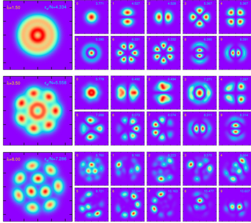
Figure 3. Hartree-Fock ground states of N_{e(h)} = 10 electrons and holes in a coupled (mass symmetric) bilayer system indicating a phase transition from a Fermi liquid to strongly coupled state upon increase in e-h separation d = \lambda \times 12\pi\epsilon\hbar^2/(e^2m_{e(h)}) and \lambda = 1.5, 3.5 , and 8.0 (from top to bottom). Left: accumulated N -particle density \rho^{e(h)}(r) . Right: corresponding densities of the 10 energetically lowest single-particle orbitals \rho_i^{e(h)}(r) (identical for electrons and holes). Note that the 10 high-density spots of the N -particle density for \lambda = 8 do not necessarily correspond to the single particles themselves as the configuration appears as a superposition of all orbitals.
